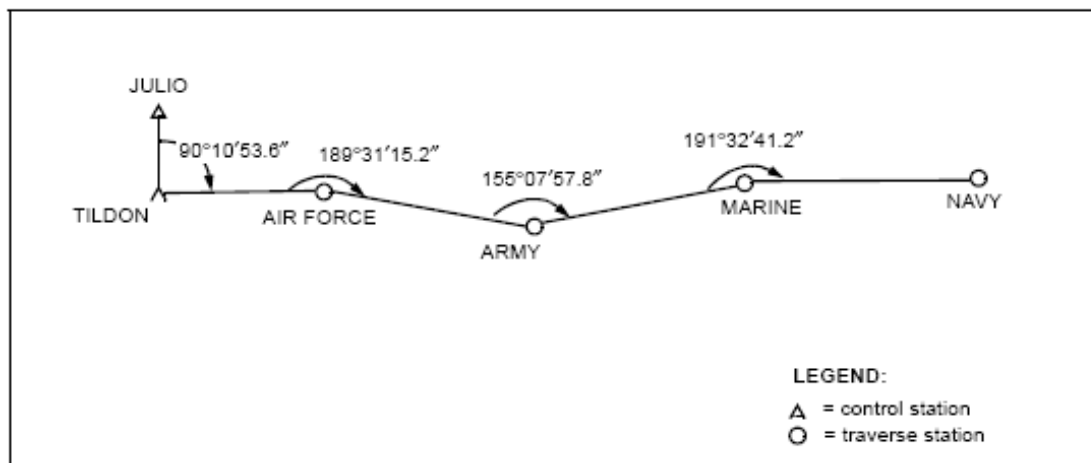
Figure 3-10. Open traverse
